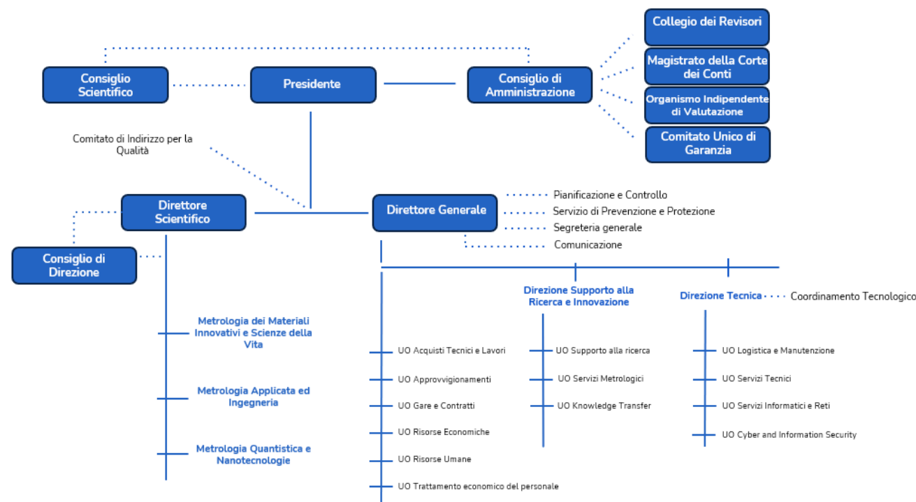
Figura 3 - Organigramma INRiM
